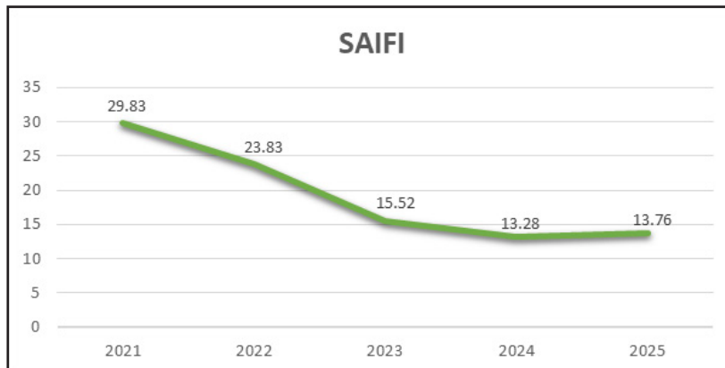
5-year Graph of SAIFI of PALECO
